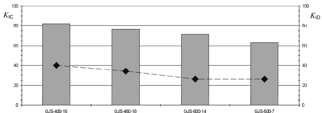
Figure F.1 — Comparison of fracture toughness as determined by K_{IC} [MPa·√m ] (grey bars) based on J_{IC} and by K_{ID} [MPa·√m ] (black diamonds) between three fully ferritic spheroidal graphite cast irons, solid solution strengthened with increasing silicon content (up to 3,8 % Si), compared to a ferritic-pearlitic spheroidal graphite cast iron of intermediate tensile strength [17] on the right
